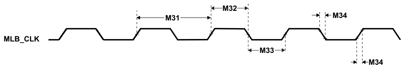
Figure 5-46. MLB_CLK Timing
